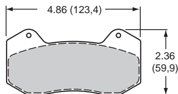
Plate 6712 P/N 150-14780K .49" Thick
