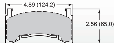
Plate D154 • P/N 150-14778K Inner/Outer .52" Thick
