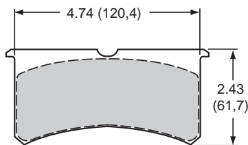
Plate 7416 / 7420 P/N 150-14772K / 150-14773K .65" / .80" Thick
