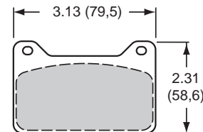
Plate 7912 P/N 150-14781K .49" Thick
