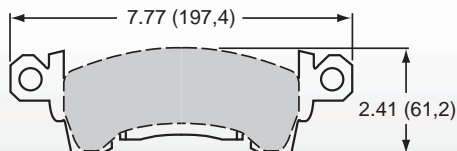
Plate D52 • P/N 150-14777K Inner .58" Thick, Outer .52" Thick
