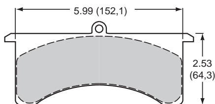
Plate 7520 P/N 150-14774K .80" Thick
