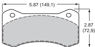
Plate 6617 / 6620 P/N 150-14779K / 150-14782K .67" / .80" Thick
