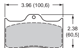
Plate 7112 P/N 150-14771K .49" Thick
