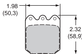
Plate 6812 P/N 150-14770K .50" Thick
