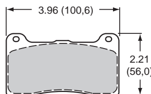
Plate 7812 / 7816 P/N 150-14775K / 150-14776K .49" / .60" Thick
