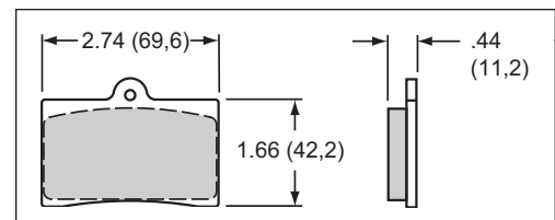
GP320 Caliper, Type 6211 Pad Dimensions
