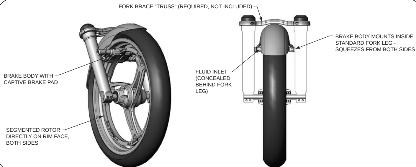
Stealth Brake System Major Components
