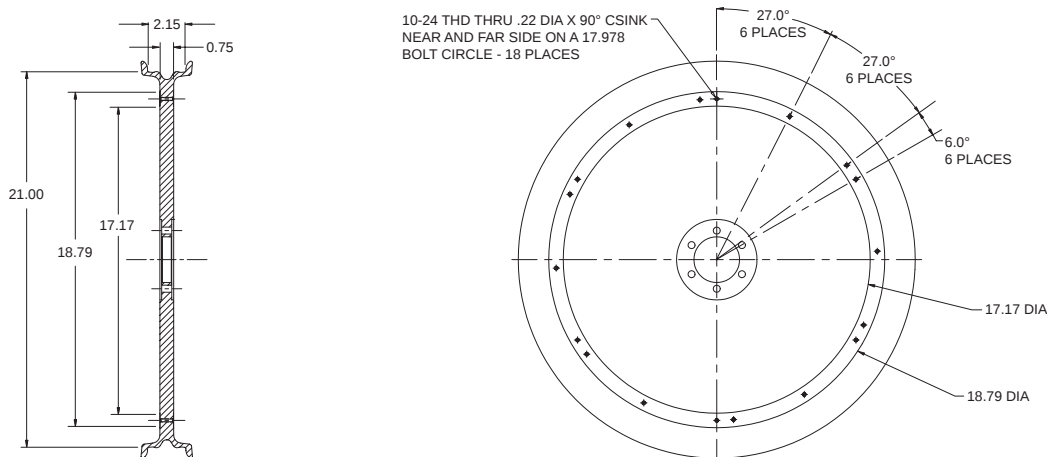
Wilwood Stealth Brake System Wheel Blank Diagram
